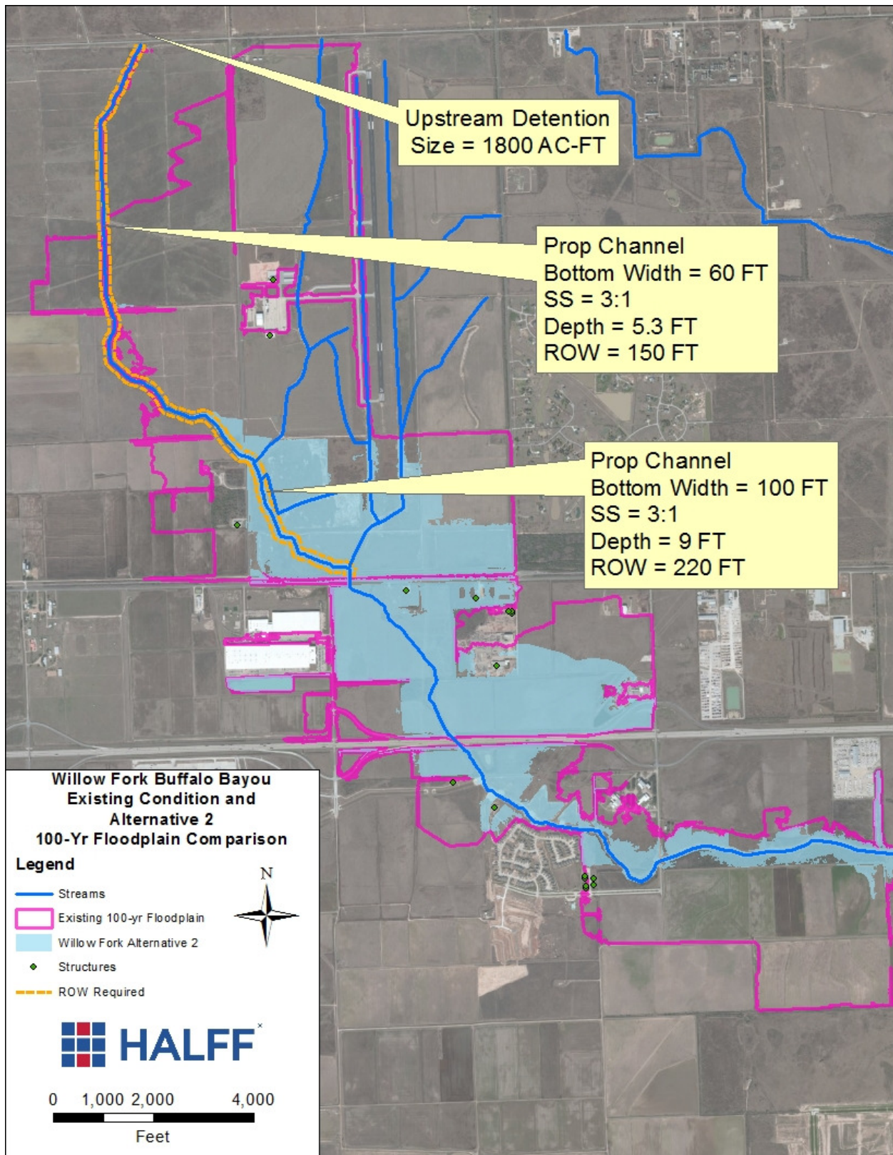
Figure B13: 100-yr Floodplain comparison between existing and Alternative 2 (Willow Fork)
