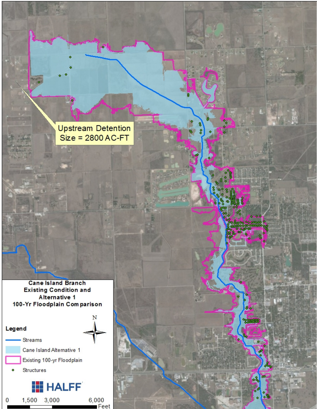
Figure B1: 100-yr Floodplain comparison between existing and Alternative 1 (Cane Island Branch)
