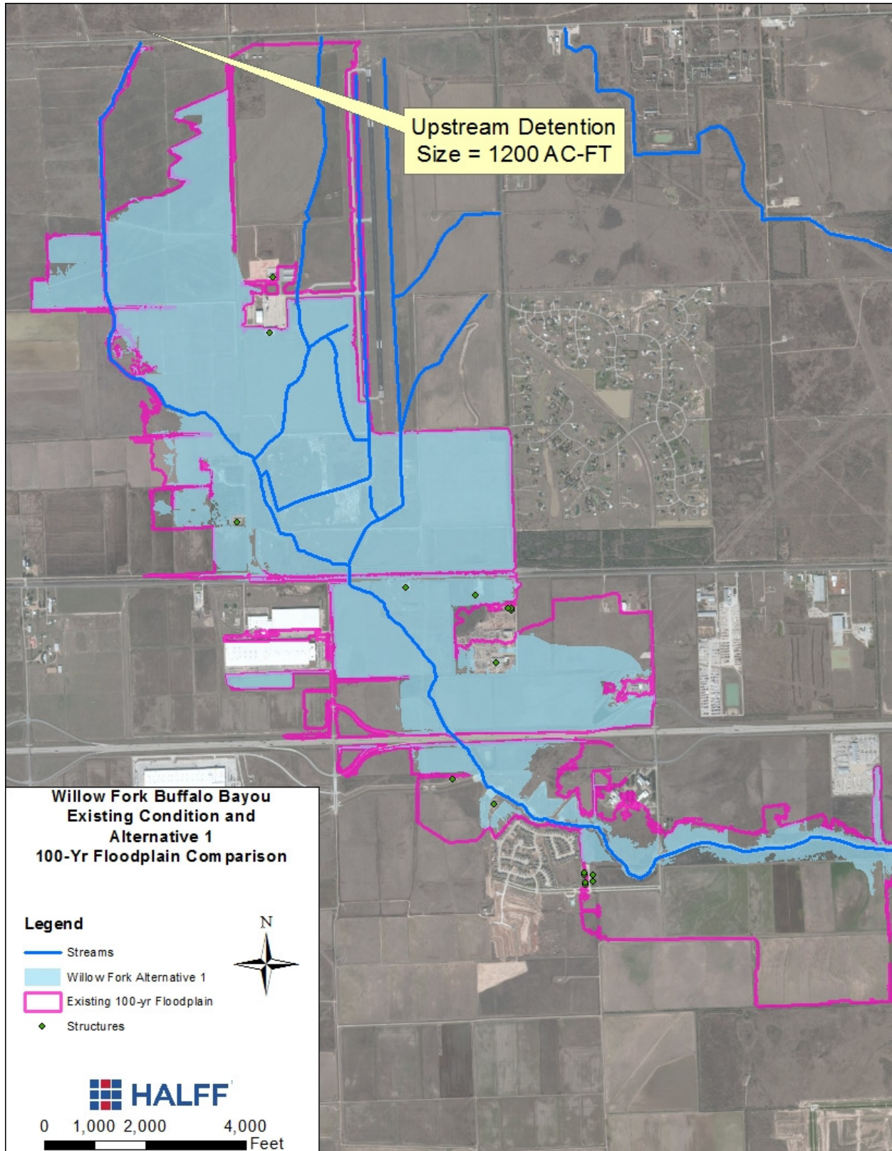
Figure B11: 100-yr Floodplain comparison between existing and Alternative 1 (Willow Fork)
