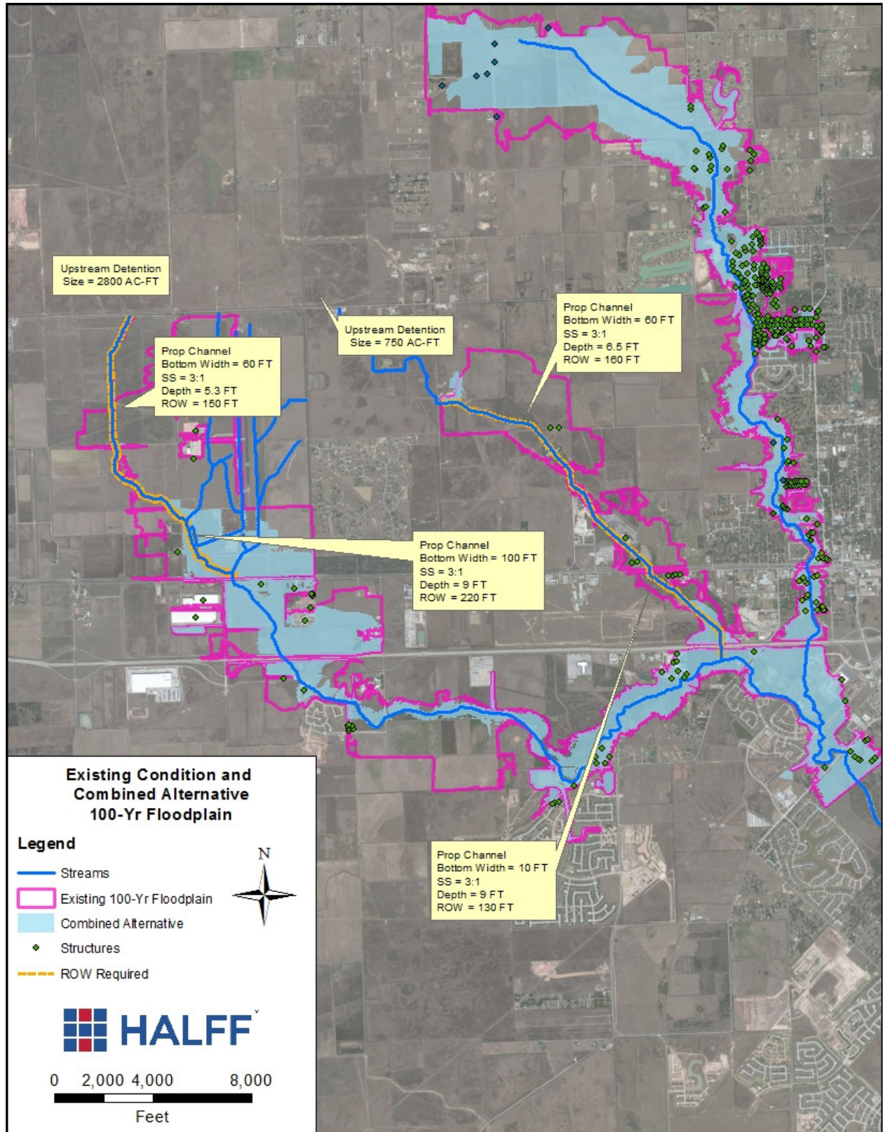
Figure B15: 100-yr Floodplain comparison between existing and Combined Alternative
