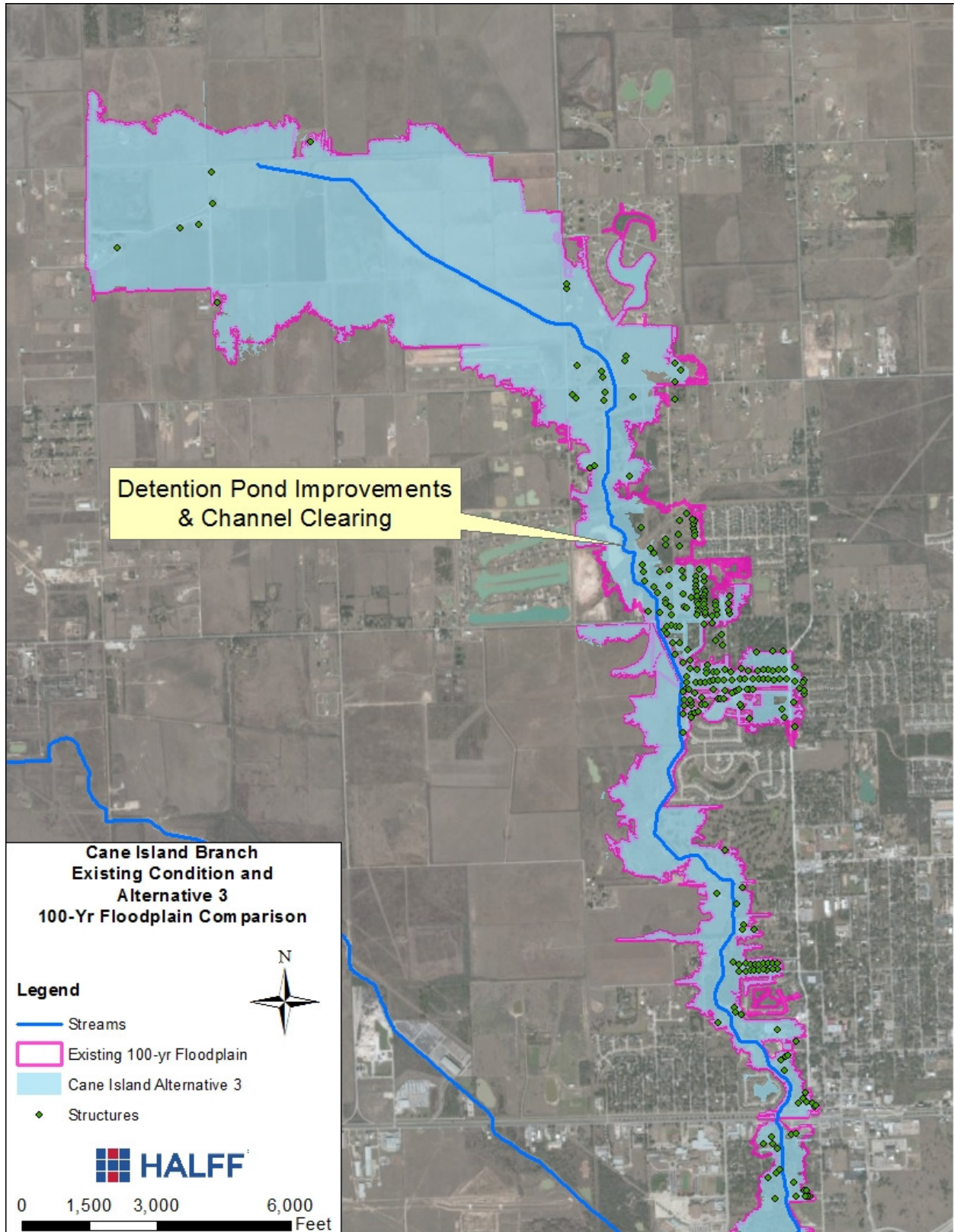
Figure B5: 100-yr Floodplain comparison between existing and Alternative 3 (Cane Island Branch)
