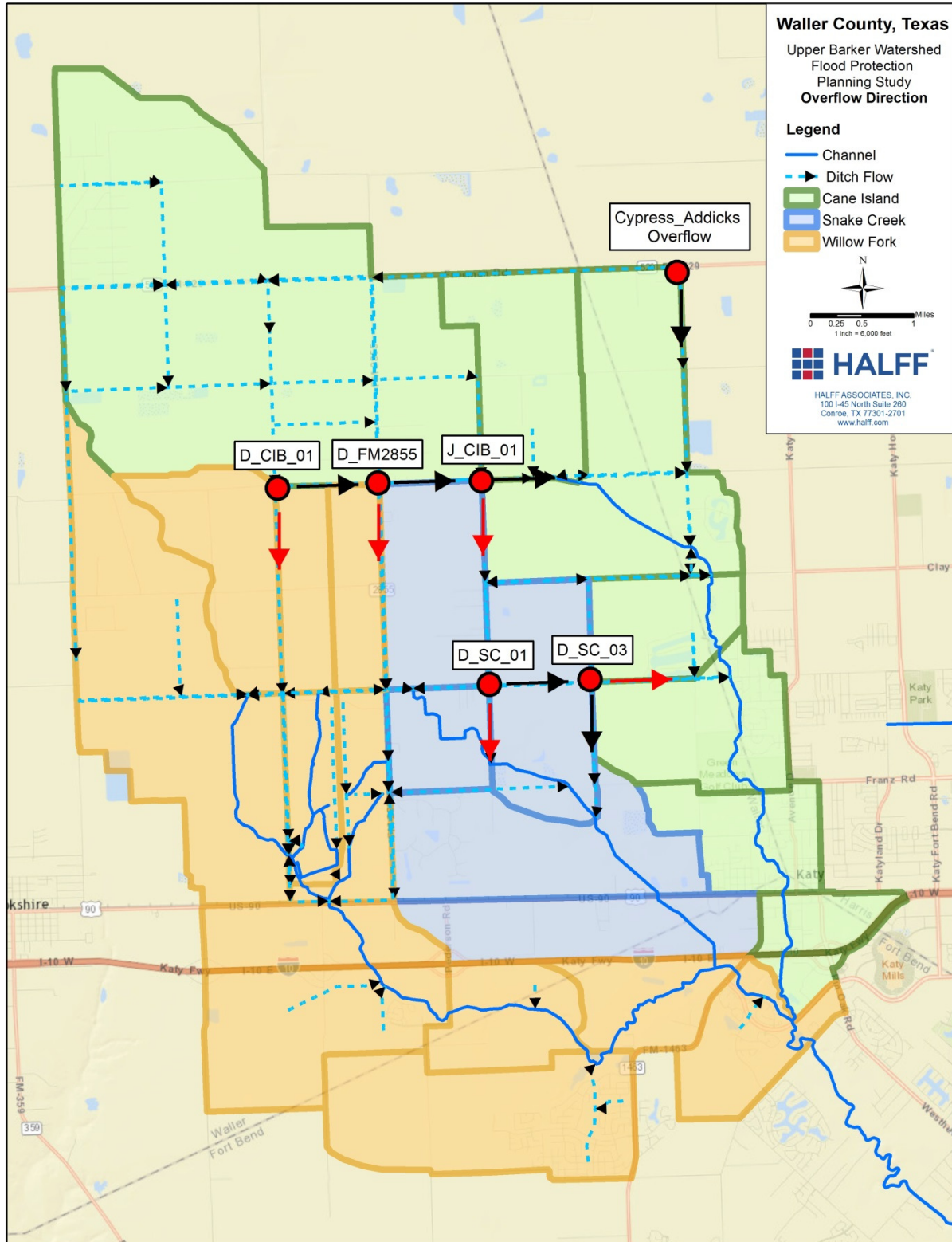
Figure A3: Flow Diversions to Represent Overflow
