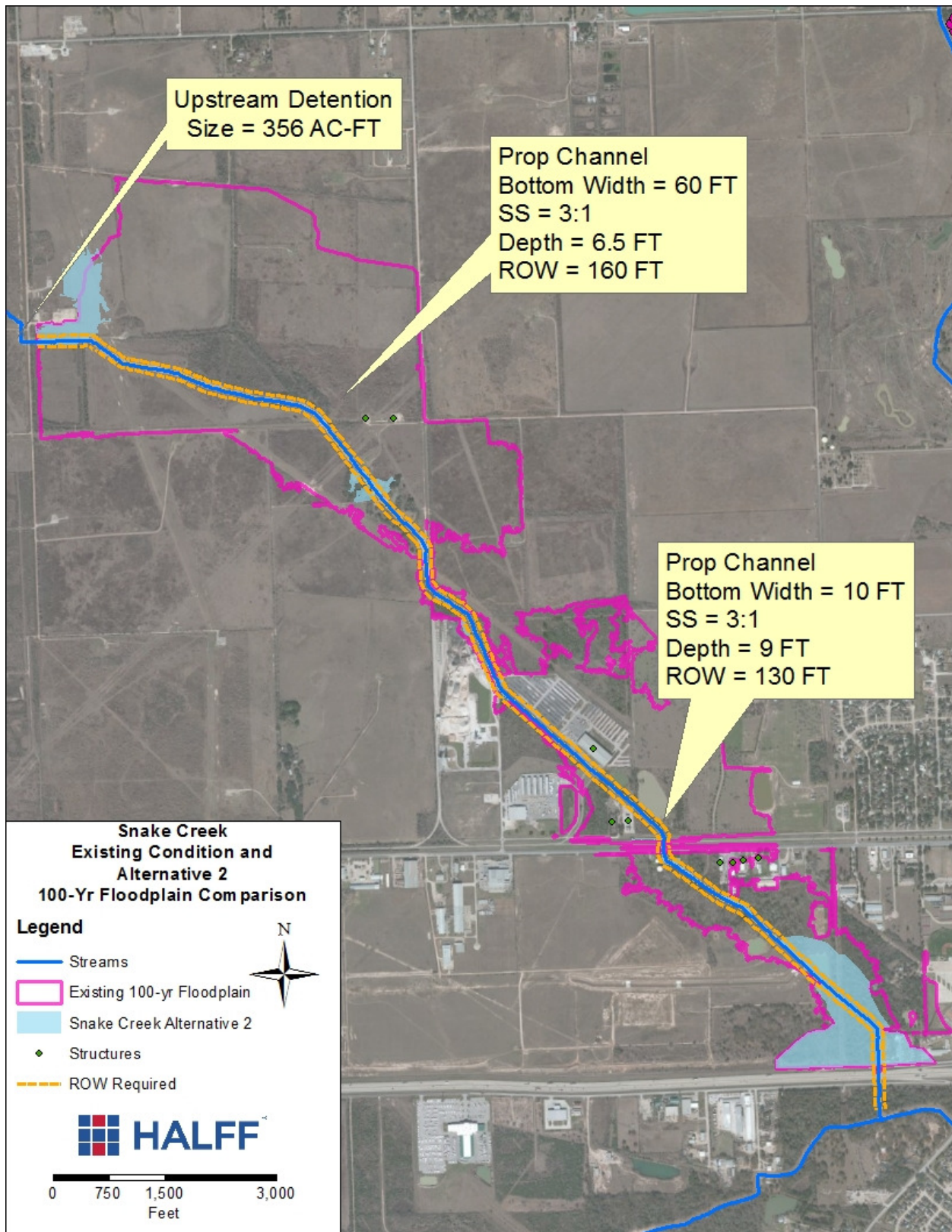
Figure B9: 100-yr Floodplain comparison between existing and Alternative 2 (Snake Creek)
