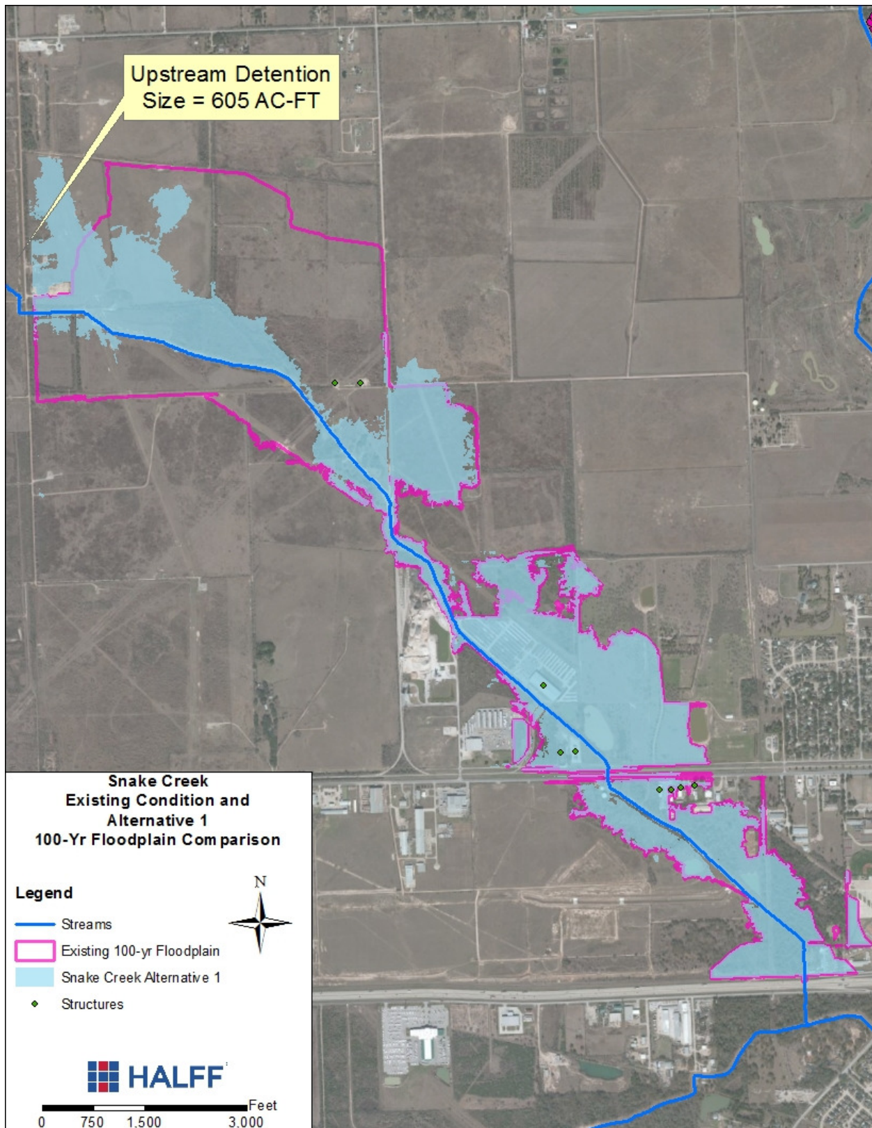
Figure B7: 100-yr Floodplain comparison between existing and Alternative 1 (Snake Creek)
